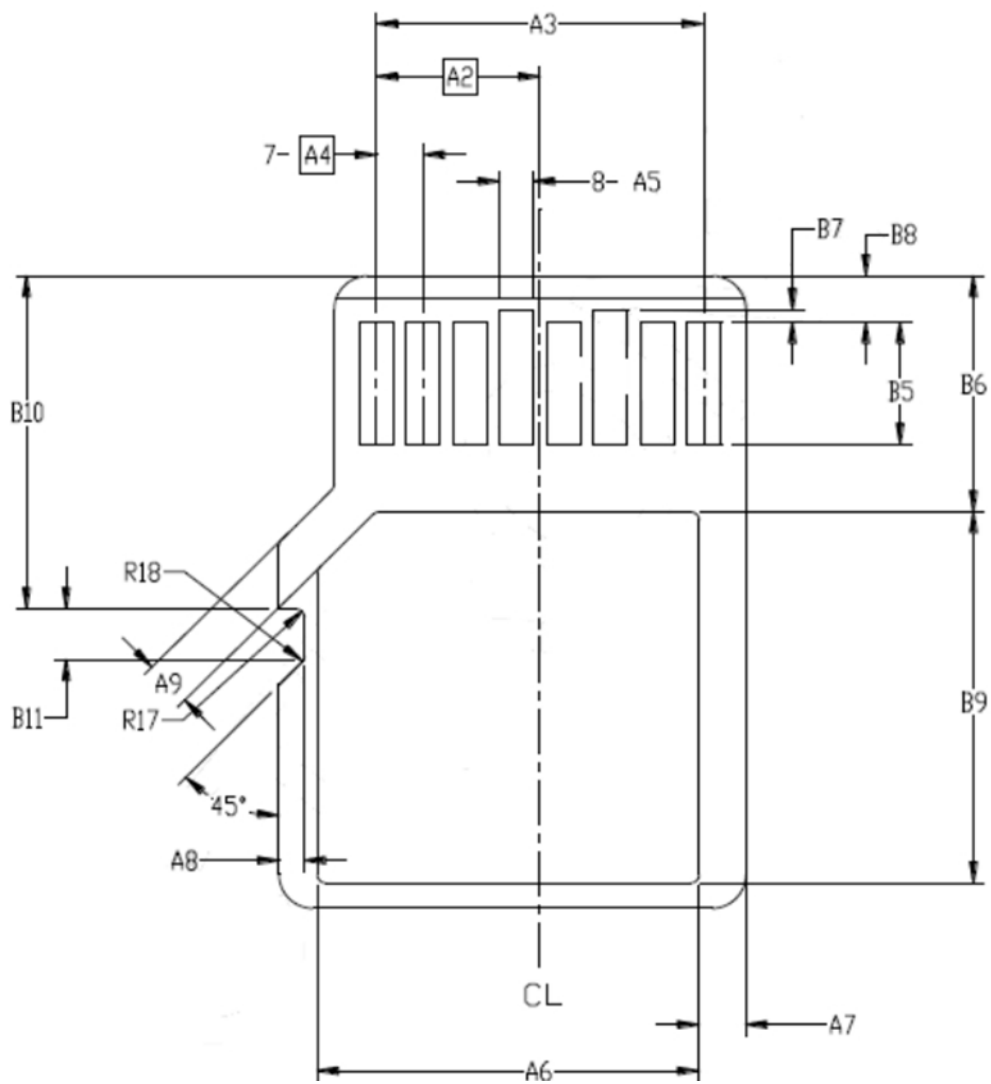
Figure 11: Bottom View
