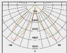
No: 1066-55W LED S Lumileds LED 55W 5101lm Clear Glass 90° symmetrical Class I, IP65
