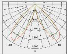
No: 1066-30W LED S Lumileds LED 30W 2924lm Clear Glass 90° symmetrical Class I, IP65
