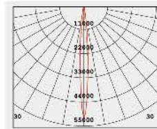
No:3109A-G12 N16 70W G12 70W HID 1424lm Clear Glass 16.00° Adjustable lampholder Class I, IP67
