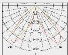
No: 1066-100W LED S Lumileds LED 100W 8056lm Clear Glass 90° symmetrical Class I, IP65
