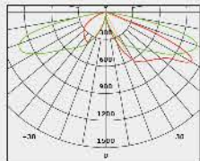
No: 1066-30W LED A Lumileds LED 30W 2842lm Clear Glass 40° asymmetrical Class I, IP65
