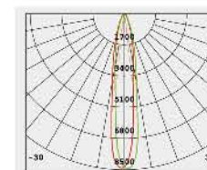
No:3110-24W LED LED 24*1W 1139lm Clear Glass 15.89° Class I, IP67
