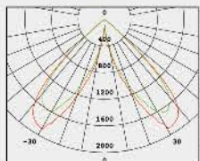
No: 1066-80W LED S Lumileds LED 80W 6759lm Clear Glass 90° symmetrical Class I, IP65
