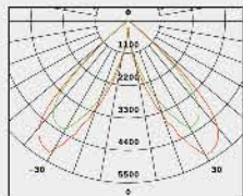
No: 1066-55W LED A Lumileds LED 55W 4949lm Clear Glass 40° asymmetrical Class I, IP65
