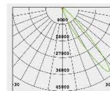
No: 3111-36W LED LED 36*1W 1629lm Clear Glass 16.44° Class I, IP67
