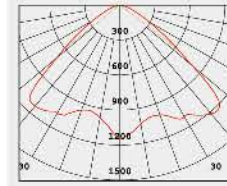
No:3109A-G12 W 70W 89W 3025lm Clear Glass 74.19° Adjustable lampholder Class I, IP67
