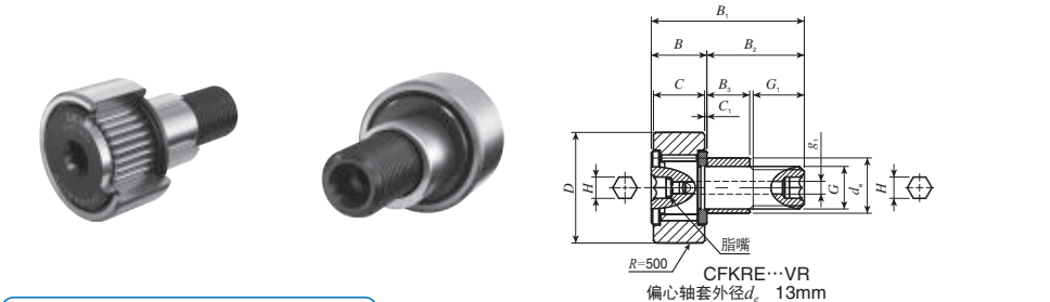
偏心轴套外径13-35mm
