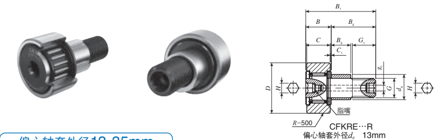
偏心轴套外径13-35mm
