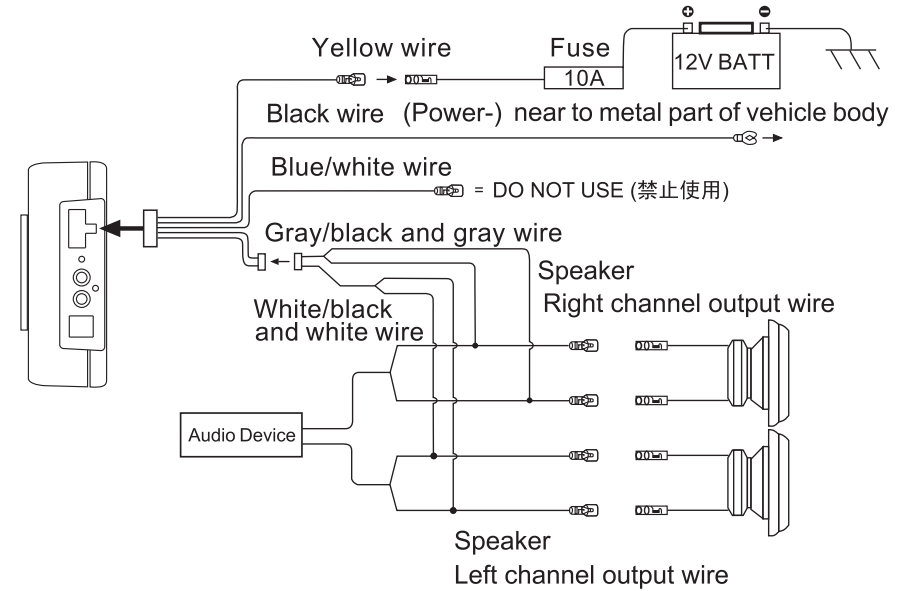
Wiring Diagram1 (High level input)
