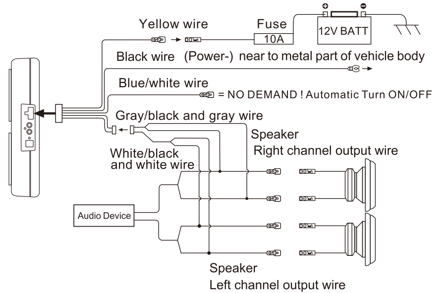
Wiring Diagram1 (High level input)
