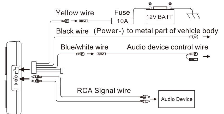
Wiring Diagram2 (Low level 'RCA' input)
