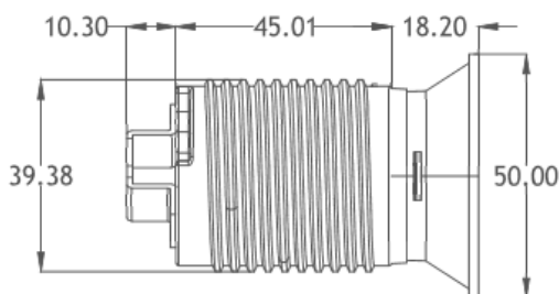
Base Type :Base Type :Conduction Body(45mm)+12° Lens+Fixer(BE)
