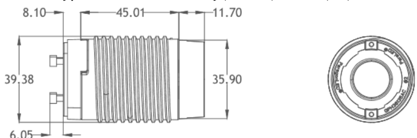
Base Type :Conduction Body(45mm)+GU24(FX)
