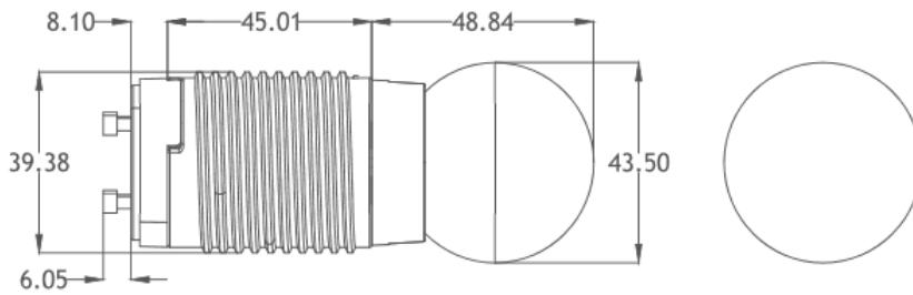
Base Type :Conduction Body(45mm)+Bulb+GU24(FA)
