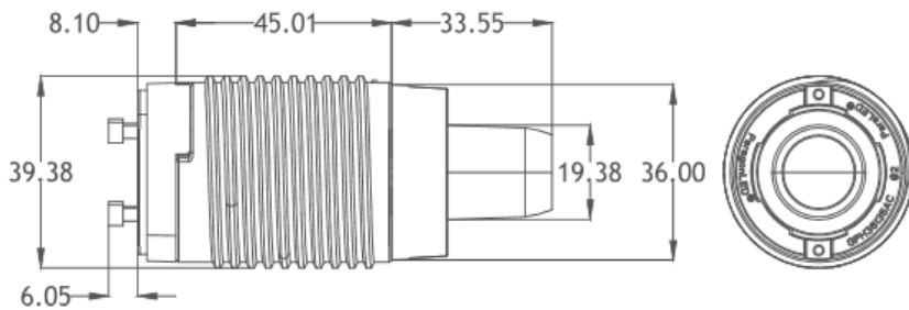
Base Type :Conduction Body(45mm)+Light guide column+GU24(FB)
