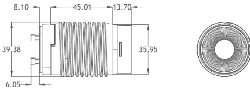
Base Type Conduction Body(45mm)+24° Lens+Fixer+GU24(FC) Conduction Body(45mm)+38° Lens+Fixer+GU24(FD)
