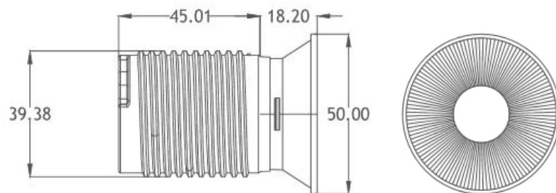
Base Type :Conduction Body(45mm)(HX)
