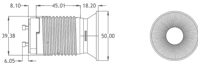
Base Type :Conduction Body(45mm)+GU24(FX)
