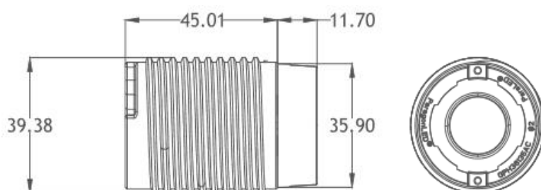
Base Type :Conduction Body(45mm)(HX)
