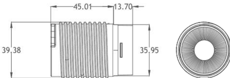
Base Type :Base Type :Conduction Body(45mm)+12° Lens(HE)
