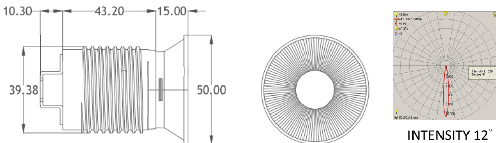
Base Type :Base Type :Conduction Body+12° Lens+Fixer(OE)
