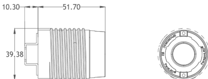
Base Type :Conduction Body+Fixer(OX)
