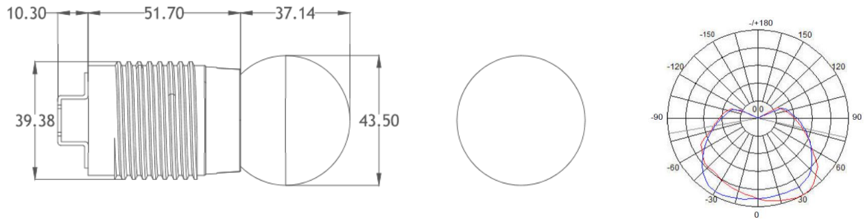
Base Type :Conduction Body+Light guide column+Fixer(OB)
