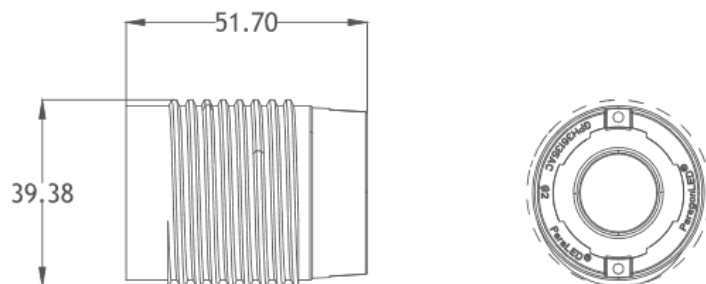
Base Type :Conduction Body(MA)
