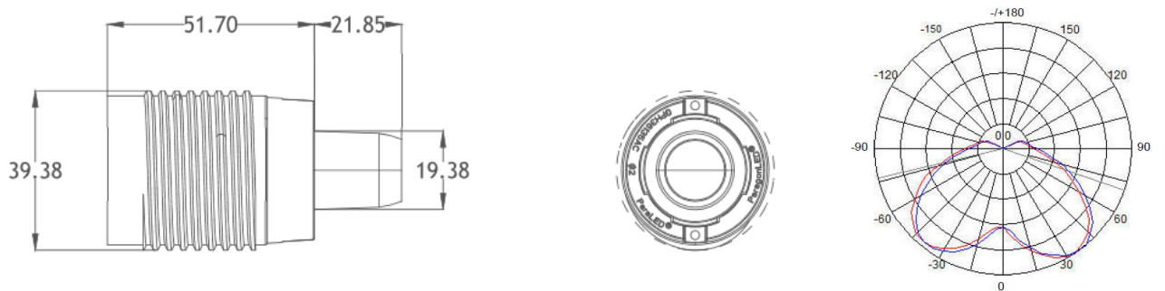
Base Type Conduction Body+24° Lens(MC) Conduction Body+38° Lens(MD)
