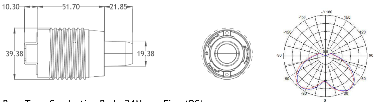
Base Type Conduction Body+24° Lens+Fixer(OC) Conduction Body+38° Lens+Fixer(OD)
