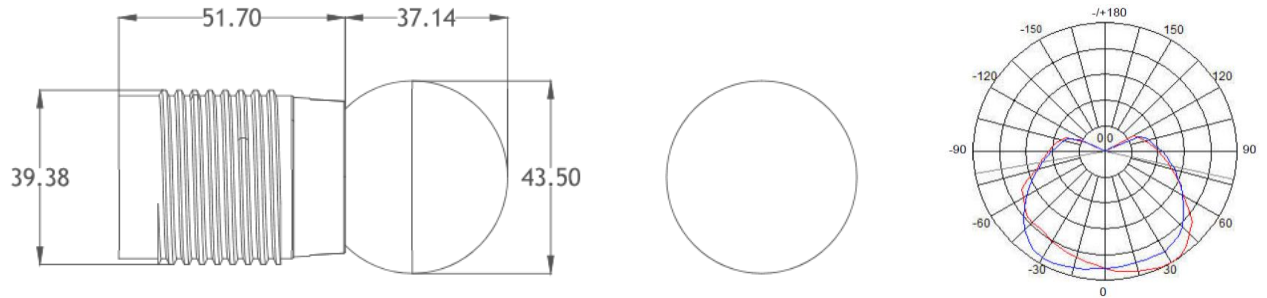
Base Type :Conduction Body+Bulb(MA)
