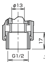
DETAIL "C"
