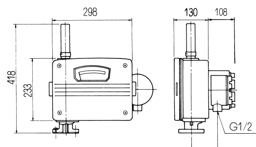
Fig. 8 : FS-115E, 1 and 2 point
