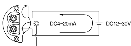
Fig. 16 : Terminal Arrangement (FS-512W and FS-512E)
