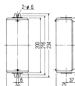
Fig. 11 : Intrinsically safe relay (For FS-115S)
