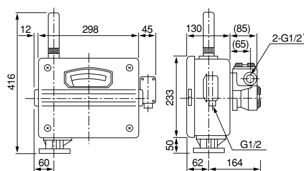
Fig. 19 : Indicator and transmitter assembly (FS-517W)
