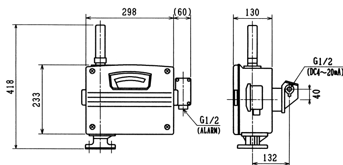
Fig. 20 : Indicator and transmitter assembly (FS-517S)
