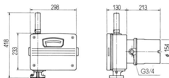
Fig. 9 : FS-115W and FS-115S, 3~6 point
