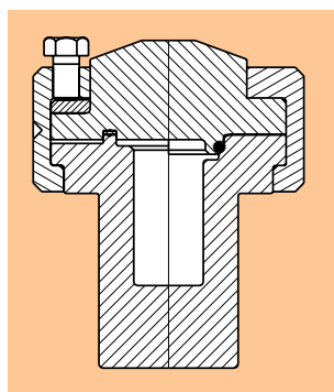
Cross Section 4791 (Showing Flat Gasket and O-ring Closure)
