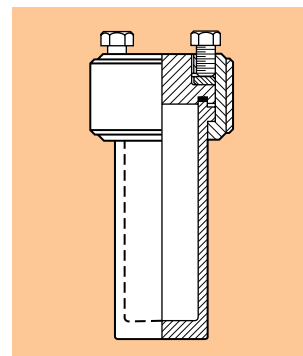
Cross Section 4750
