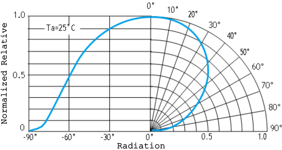
Beam Pattern
